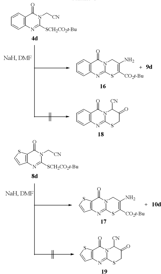
Scheme 5
